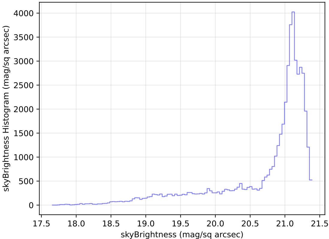
smc_lmc_v3.3_10yrs Yr 1 r band: skyBrightness Histogram
