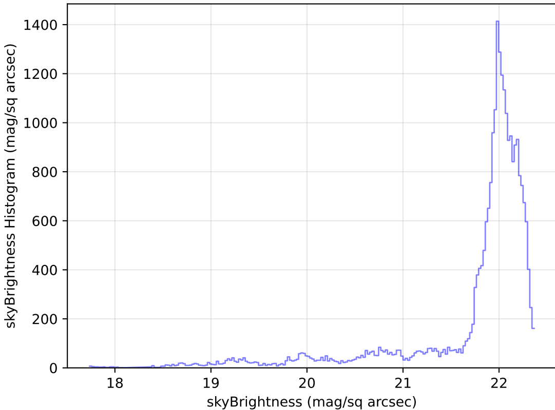
smc_lmc_v3.3_10yrs Yr 1 g band: skyBrightness Histogram
