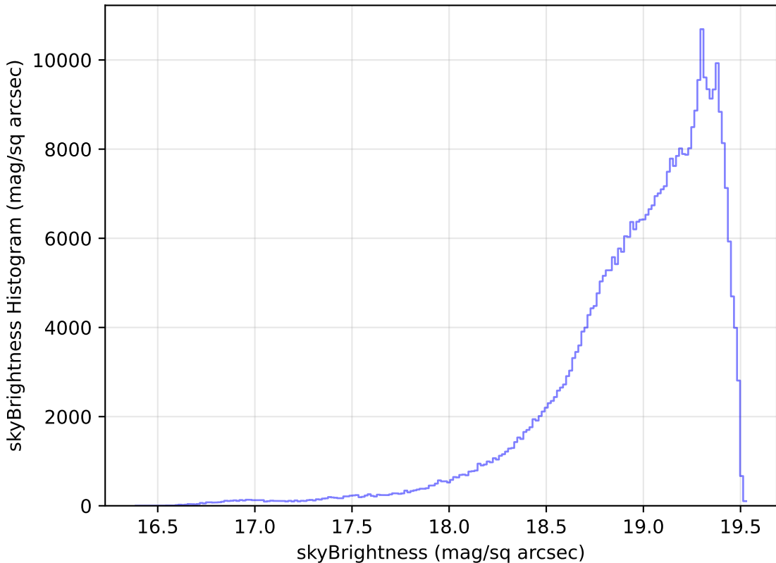
smc_lmc_v3.3_10yrs WFD z band: skyBrightness Histogram
