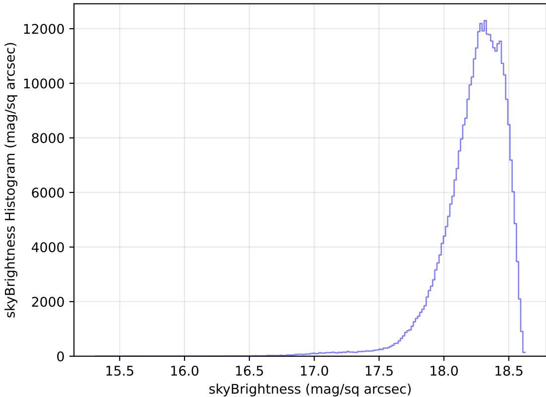
smc_lmc_v3.3_10yrs WFD y band: skyBrightness Histogram
