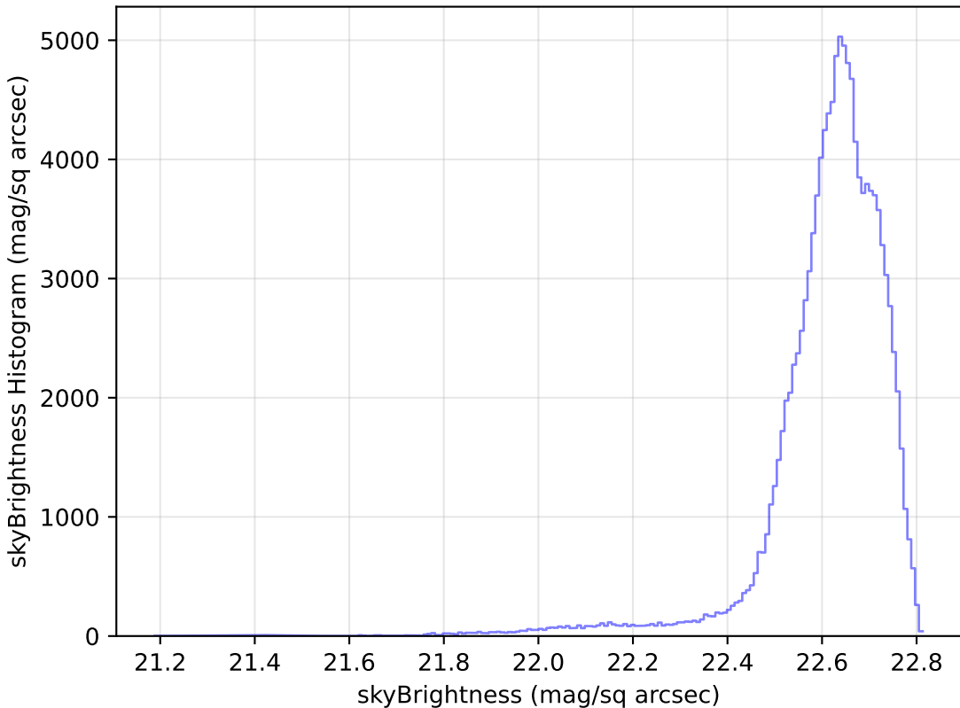
smc_lmc_v3.3_10yrs WFD u band: skyBrightness Histogram
