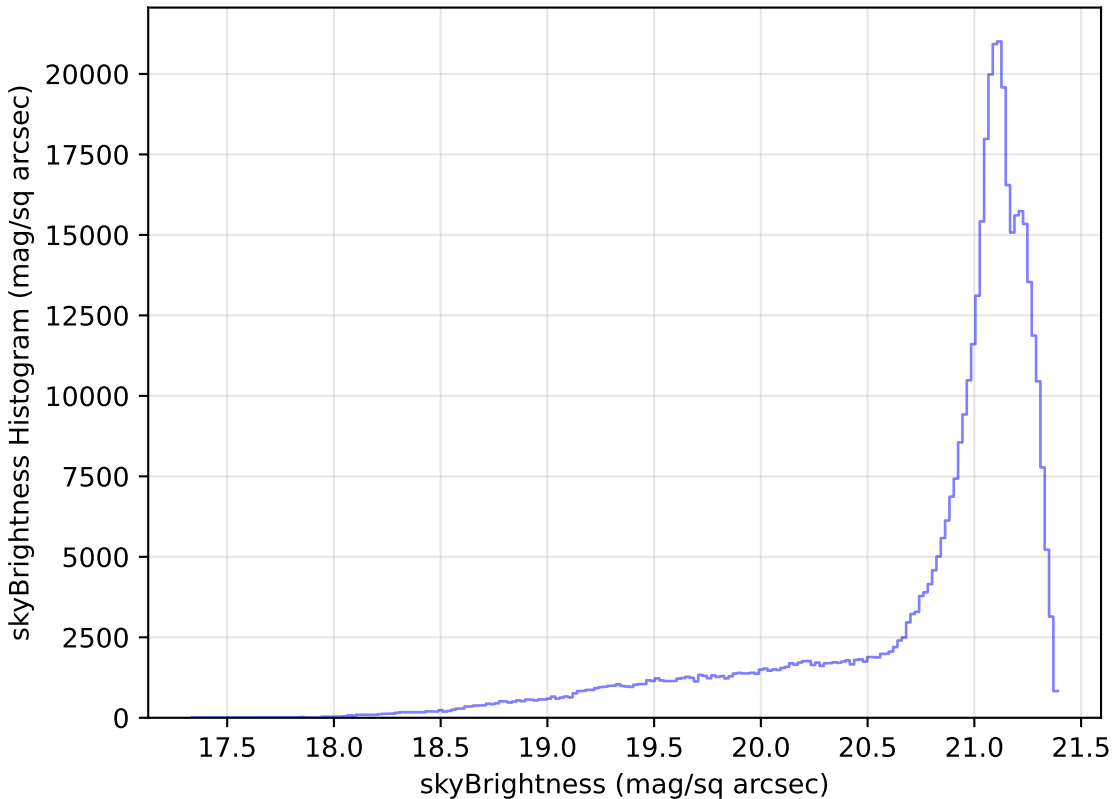
smc_lmc_v3.3_10yrs WFD r band: skyBrightness Histogram
