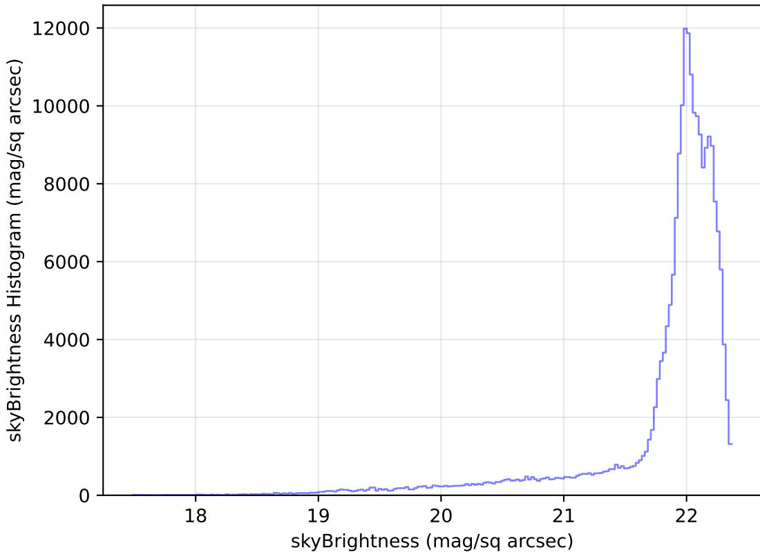
smc_lmc_v3.3_10yrs WFD g band: skyBrightness Histogram
