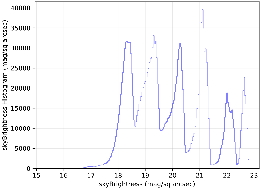
smc_lmc_v3.3_10yrs WFD all bands: skyBrightness Histogram
