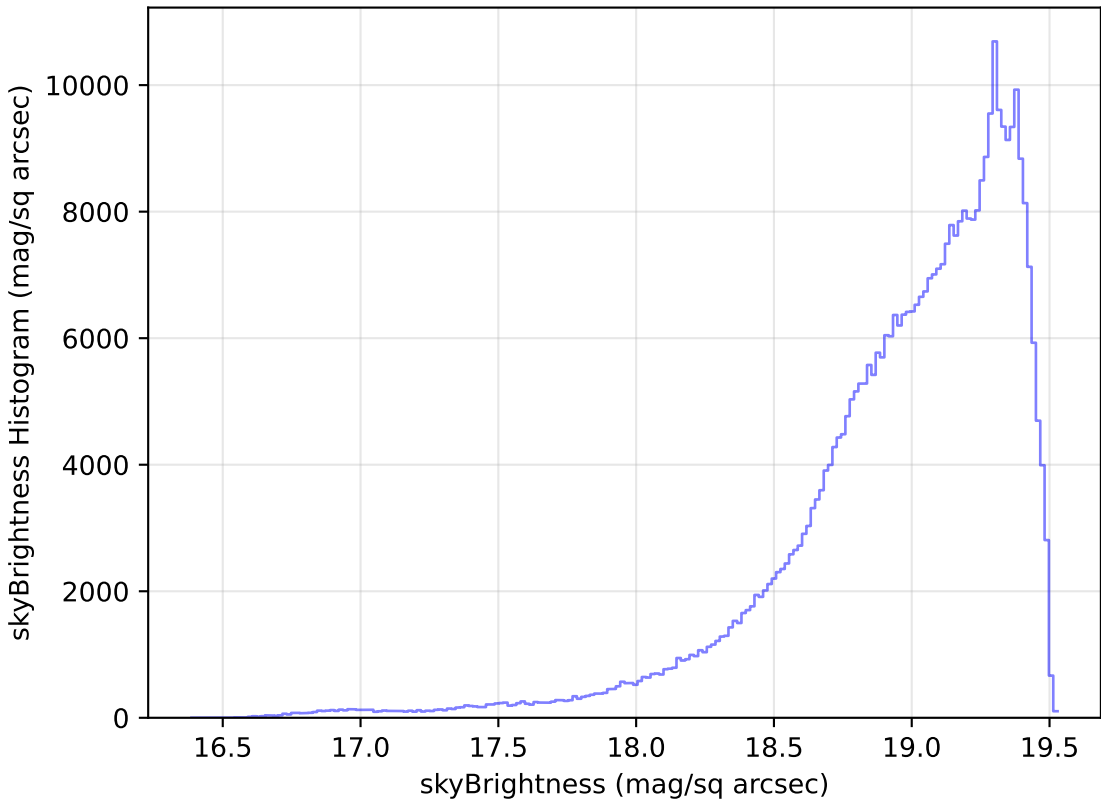
smc_lmc_v3.3_10yrs All sky z band: skyBrightness Histogram
