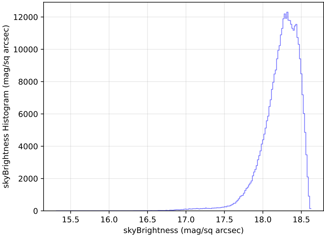
smc_lmc_v3.3_10yrs All sky y band: skyBrightness Histogram
