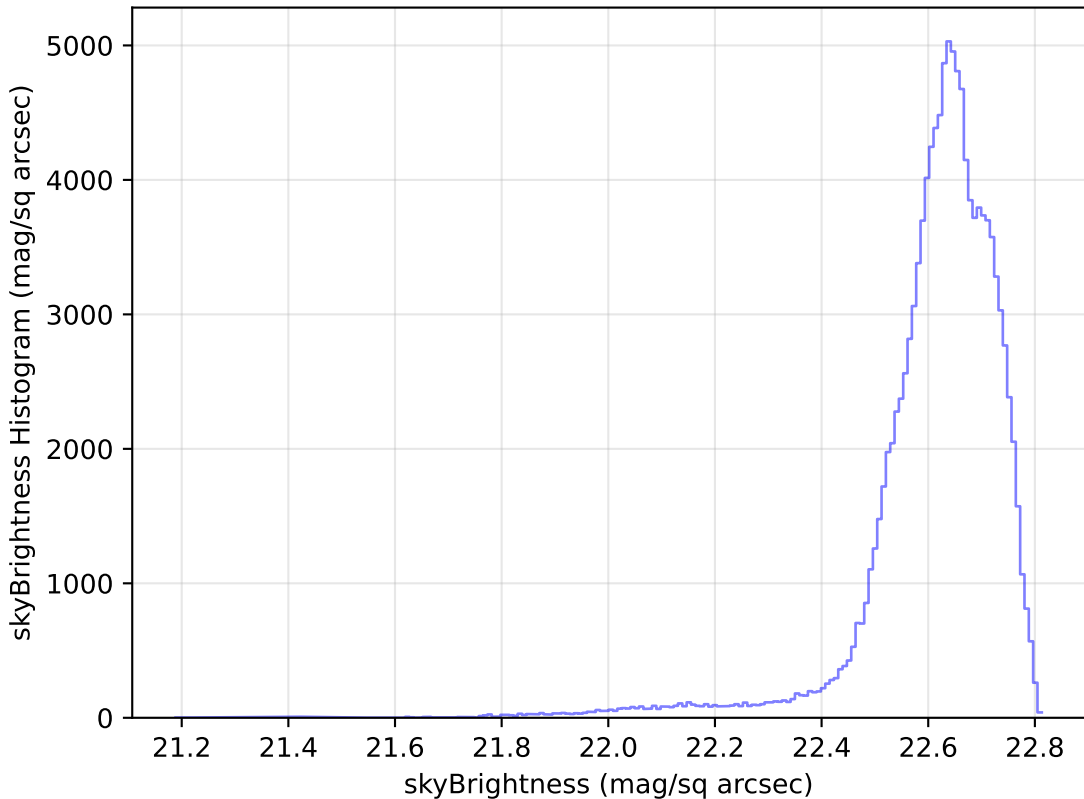
smc_lmc_v3.3_10yrs All sky u band: skyBrightness Histogram
