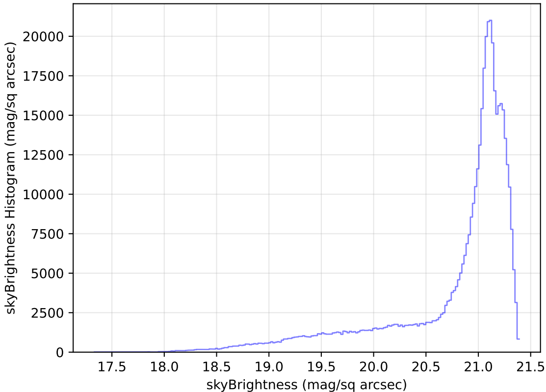
smc_lmc_v3.3_10yrs All sky r band: skyBrightness Histogram
