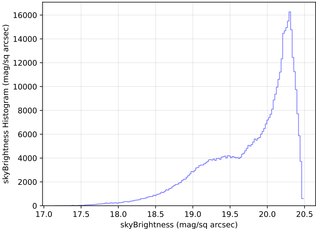
smc_lmc_v3.3_10yrs All sky i band: skyBrightness Histogram
