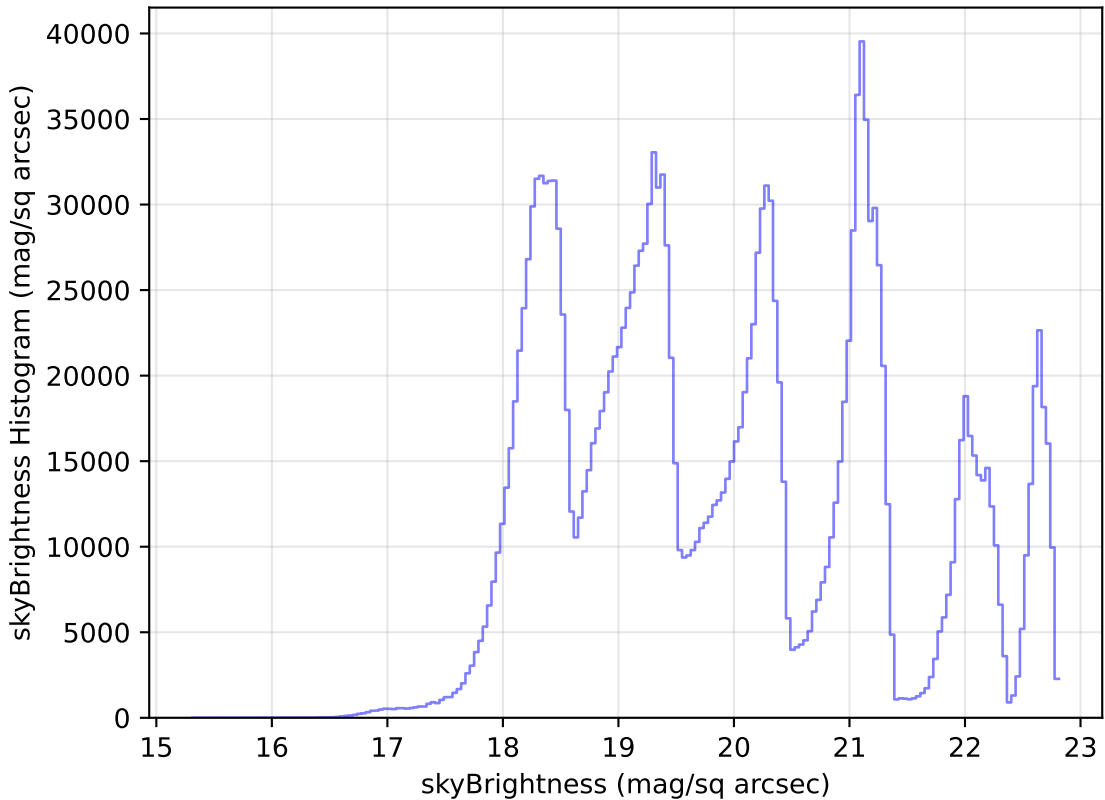
smc_lmc_v3.3_10yrs All sky all bands: skyBrightness Histogram
