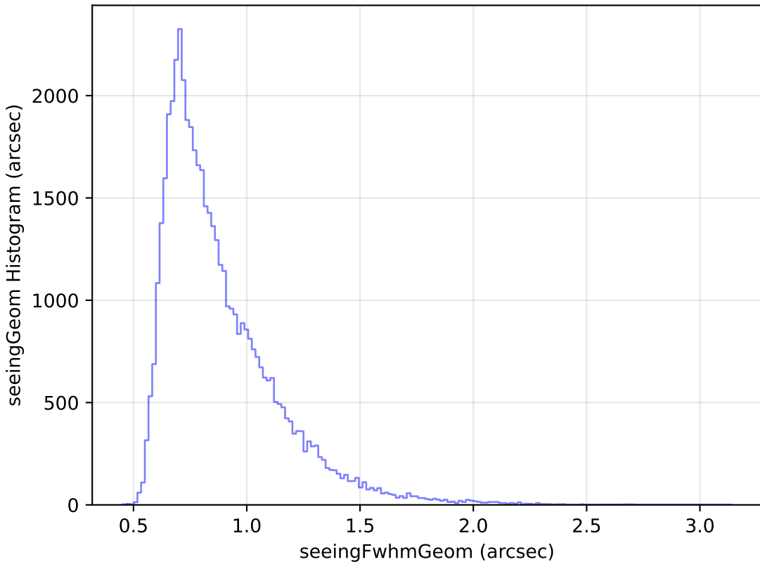
smc_lmc_v3.3_10yrs Yr 1 r band: seeingGeom Histogram
