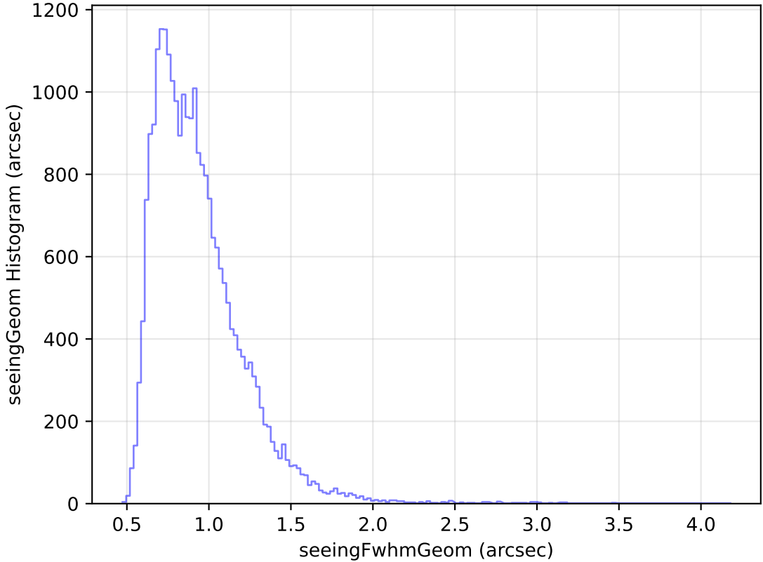
smc_lmc_v3.3_10yrs Yr 1 g band: seeingGeom Histogram
