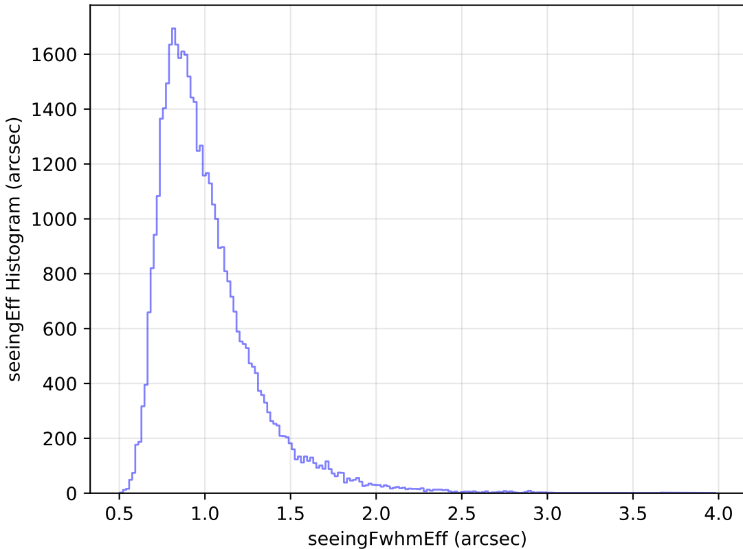
smc_lmc_v3.3_10yrs Yr 1 z band: seeingEff Histogram
