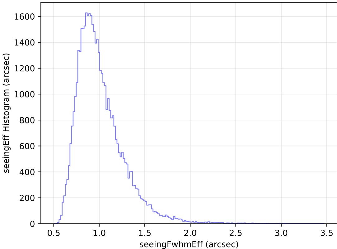
smc_lmc_v3.3_10yrs Yr 1 y band: seeingEff Histogram
