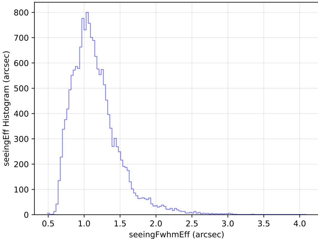
smc_lmc_v3.3_10yrs Yr 1 u band: seeingEff Histogram
