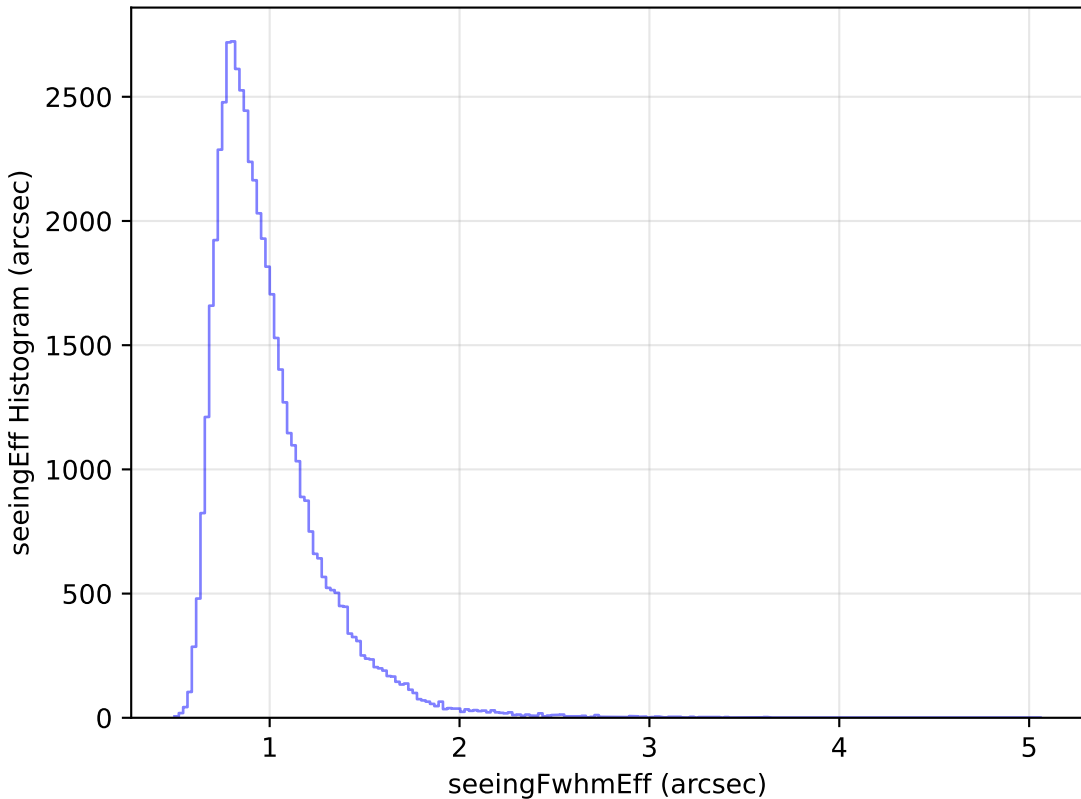
smc_lmc_v3.3_10yrs Yr 1 i band: seeingEff Histogram
