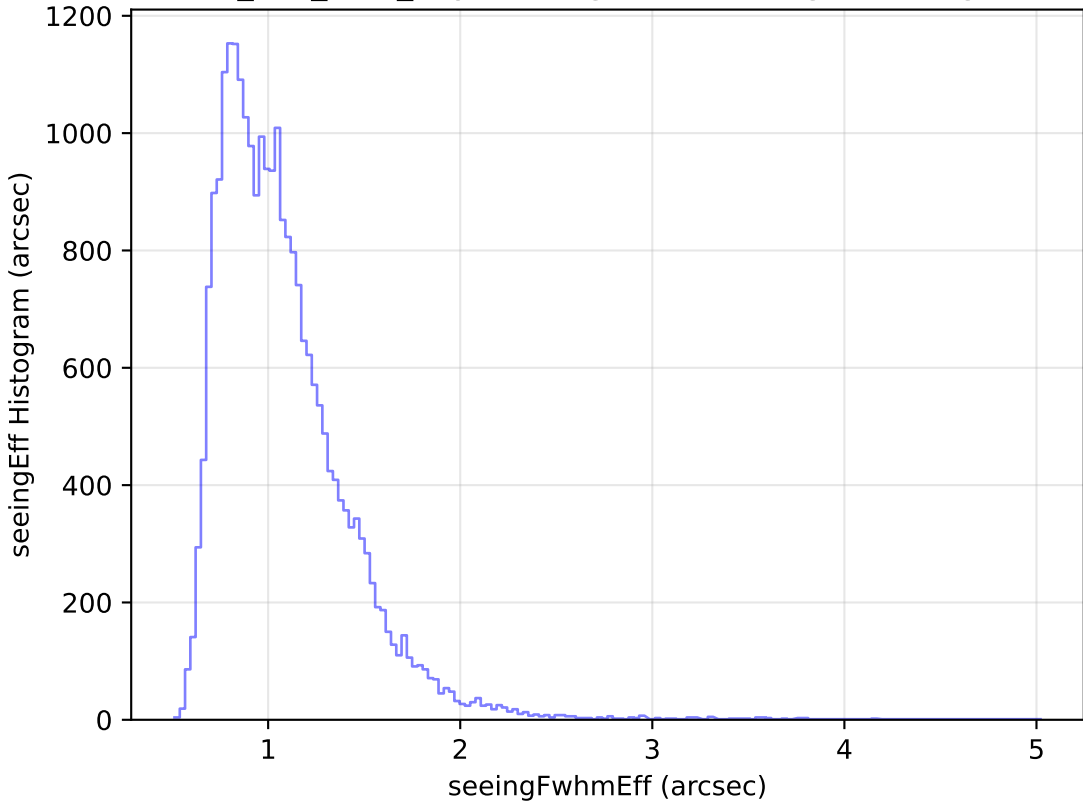
smc_lmc_v3.3_10yrs Yr 1 g band: seeingEff Histogram
