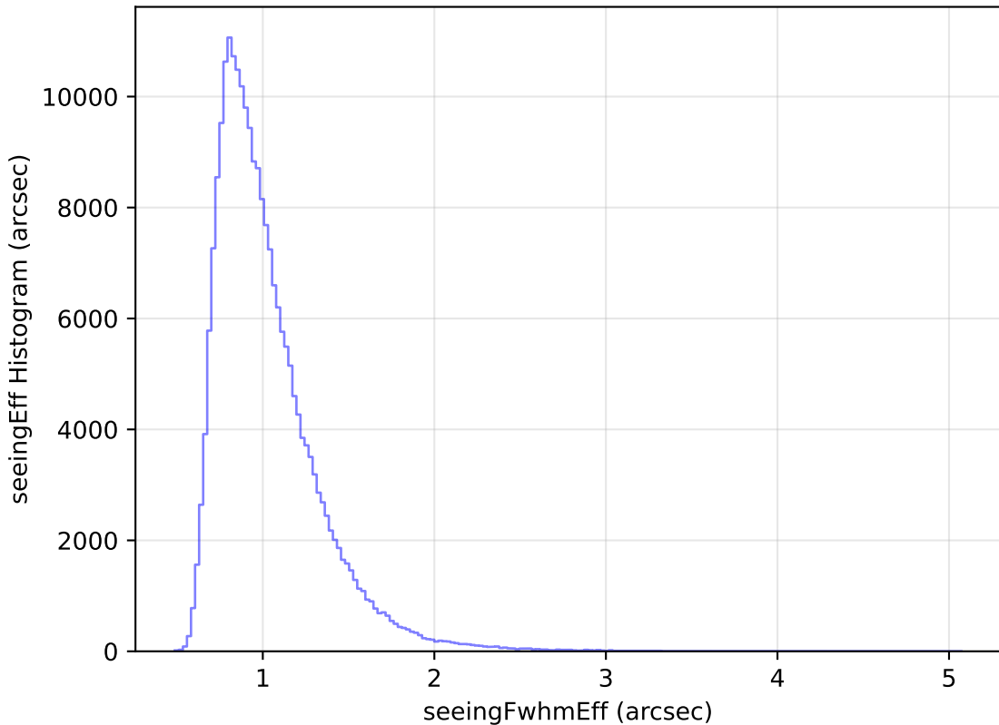
smc_lmc_v3.3_10yrs Yr 1 all bands: seeingEff Histogram
