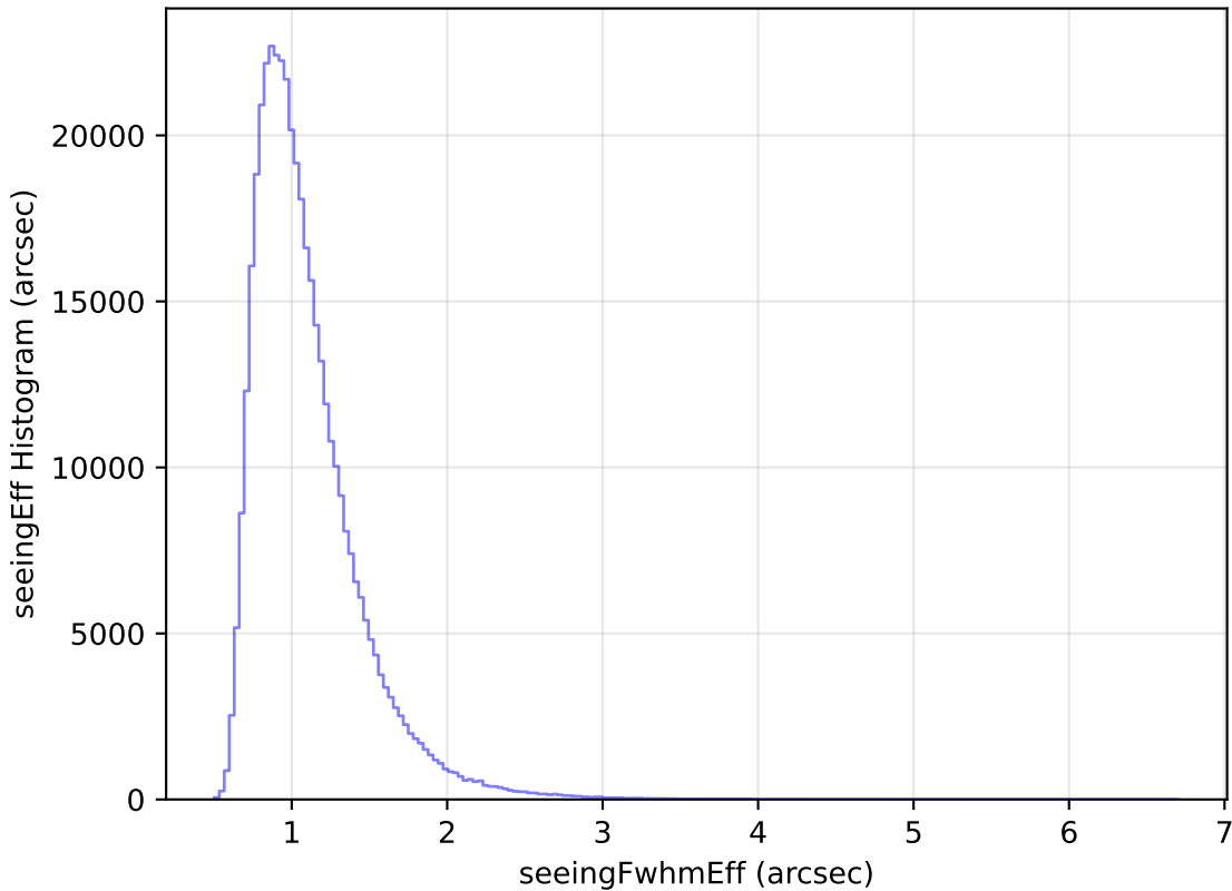
smc_lmc_v3.3_10yrs WFD z band: seeingEff Histogram
