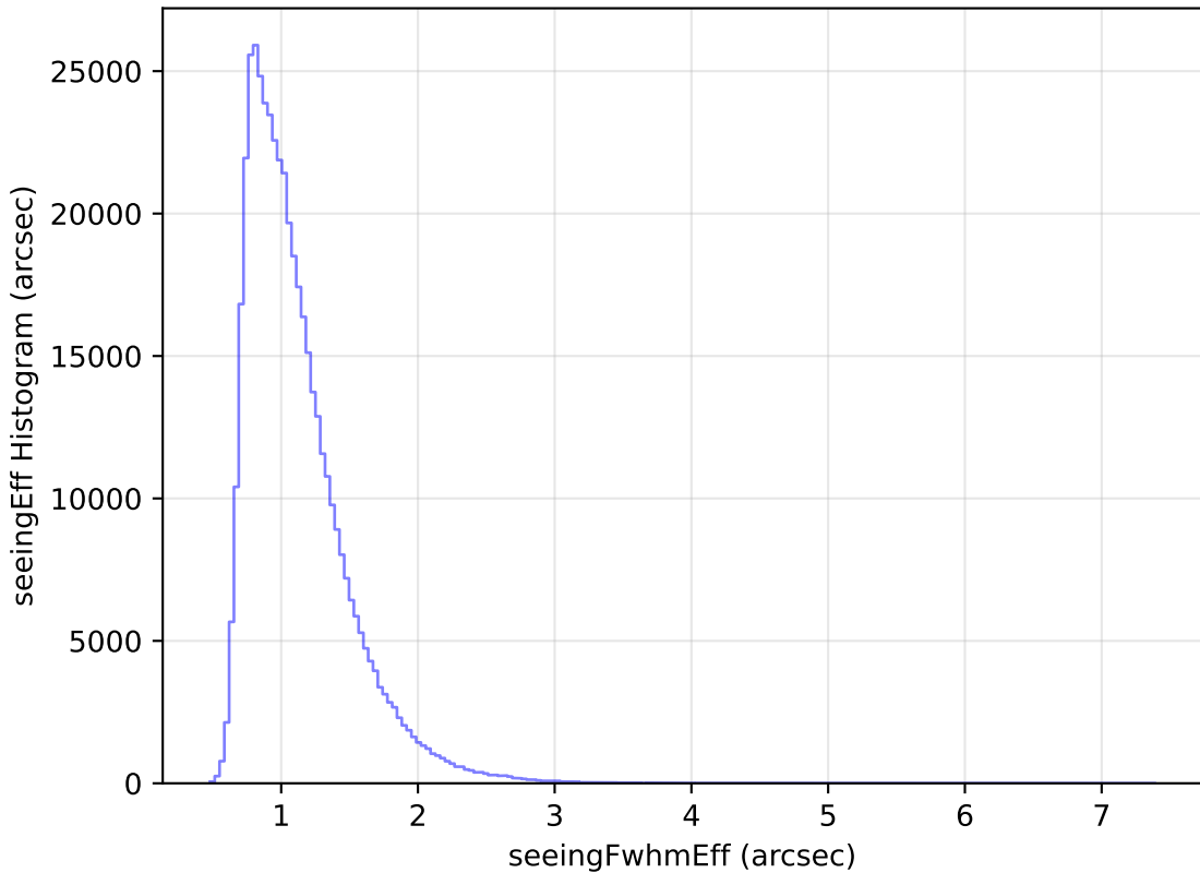
smc_lmc_v3.3_10yrs WFD r band: seeingEff Histogram
