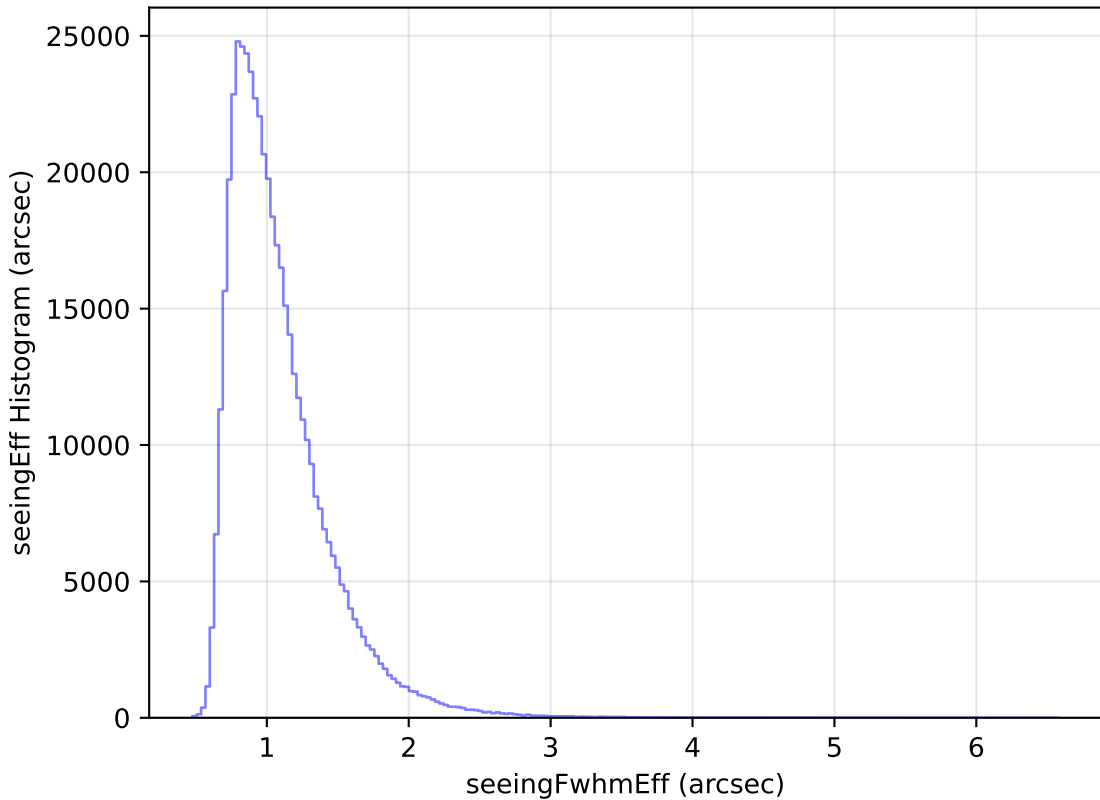
smc_lmc_v3.3_10yrs WFD i band: seeingEff Histogram
