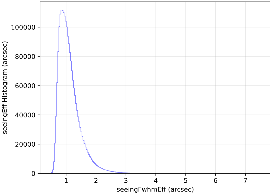
smc_lmc_v3.3_10yrs WFD all bands: seeingEff Histogram
