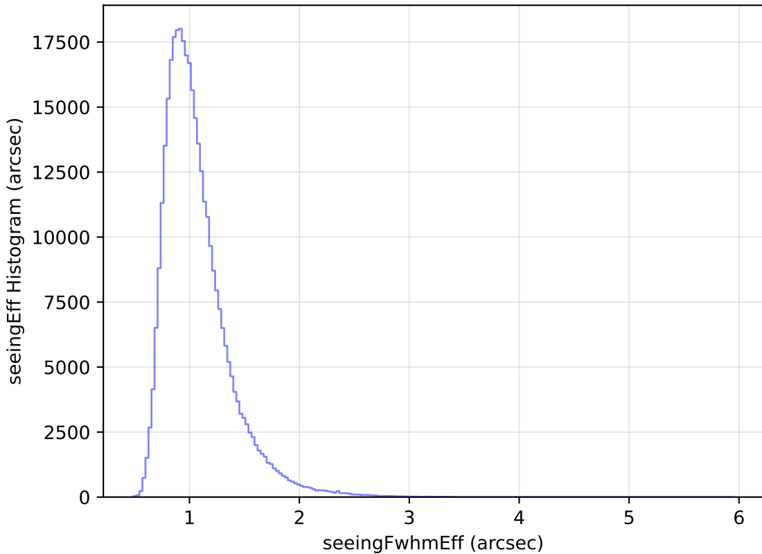
smc_lmc_v3.3_10yrs All sky y band: seeingEff Histogram
