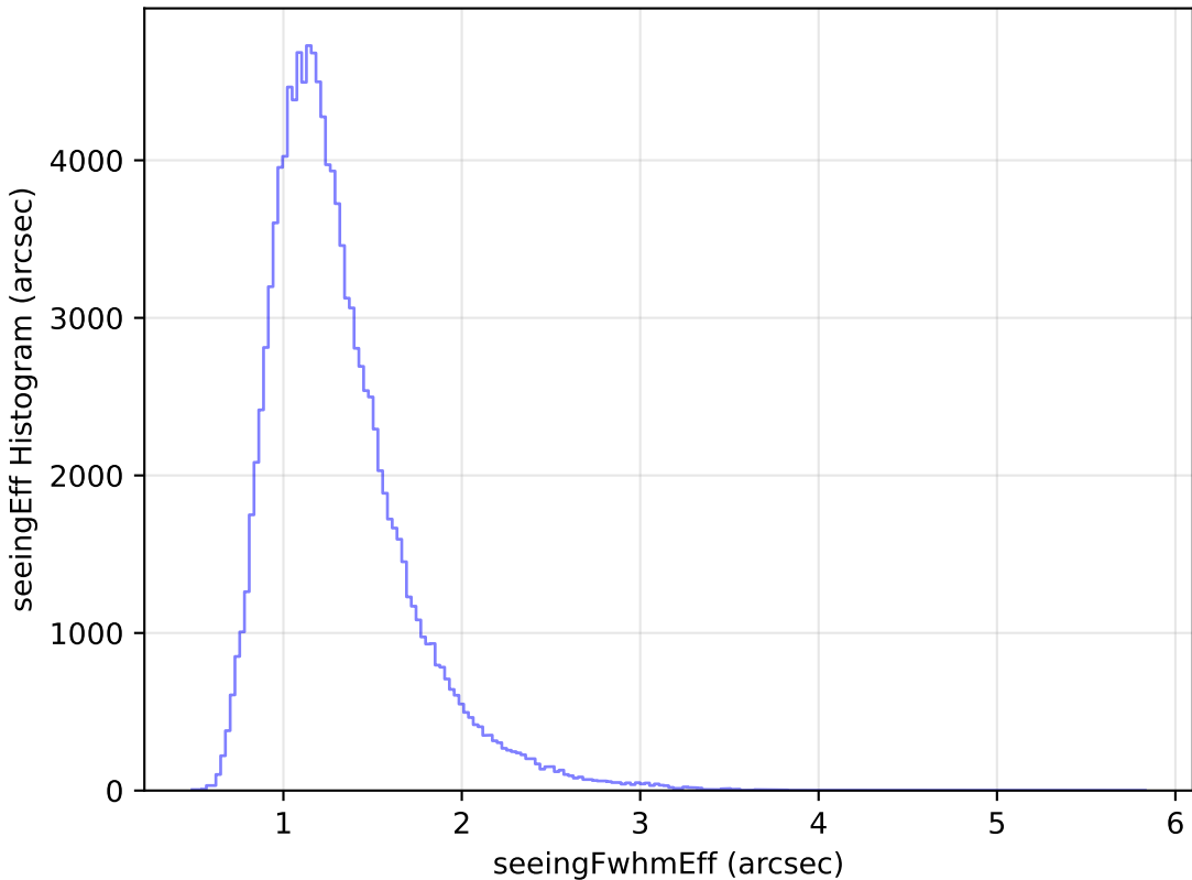
smc_lmc_v3.3_10yrs All sky u band: seeingEff Histogram
