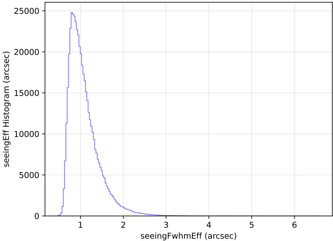
smc_lmc_v3.3_10yrs All sky i band: seeingEff Histogram
