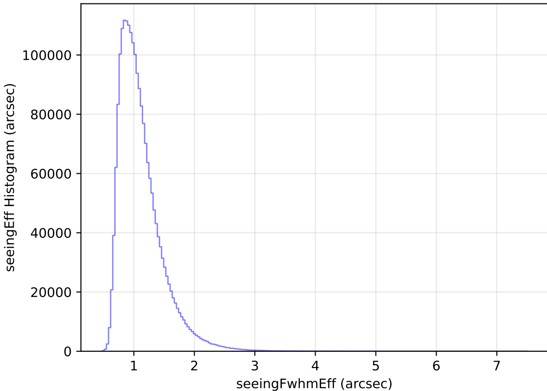
smc_lmc_v3.3_10yrs All sky all bands: seeingEff Histogram
