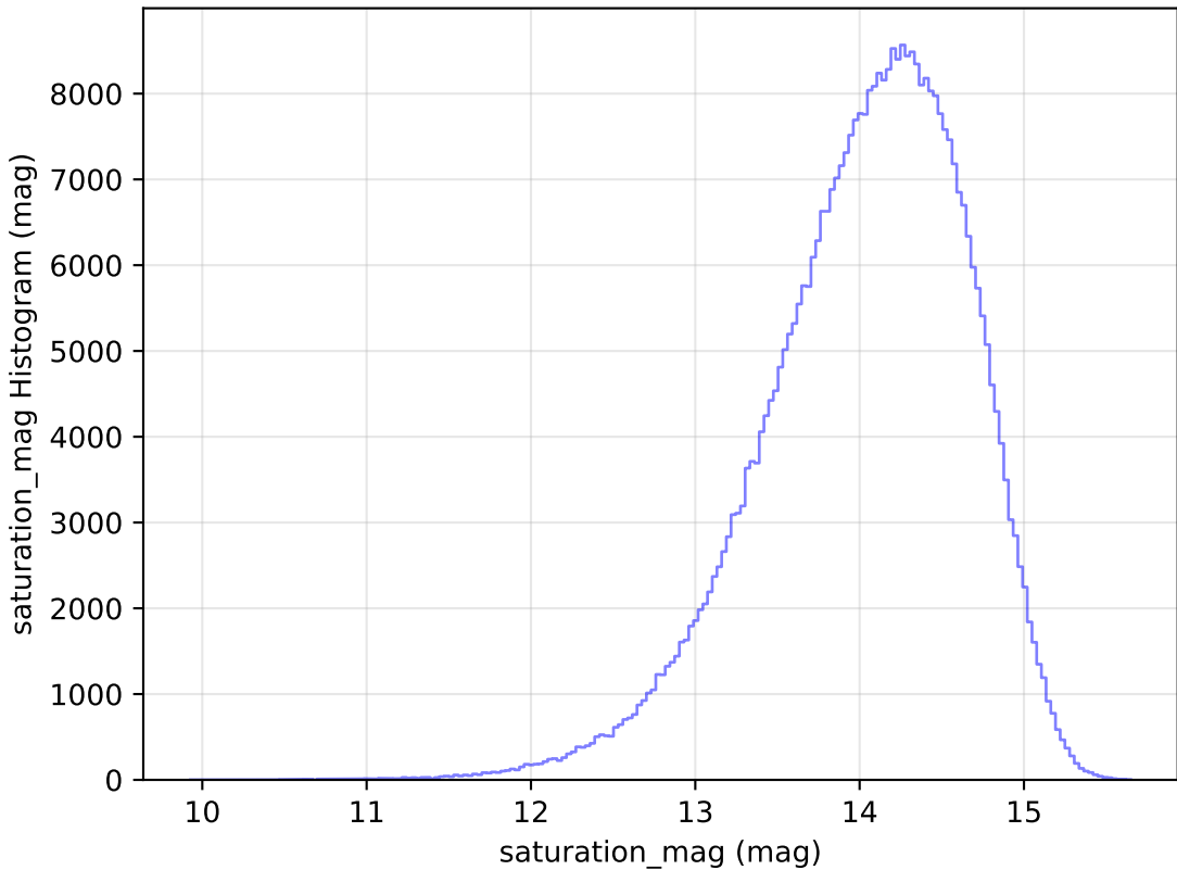
smc_lmc_v3.3_10yrs WFD z band: saturation_mag Histogram
