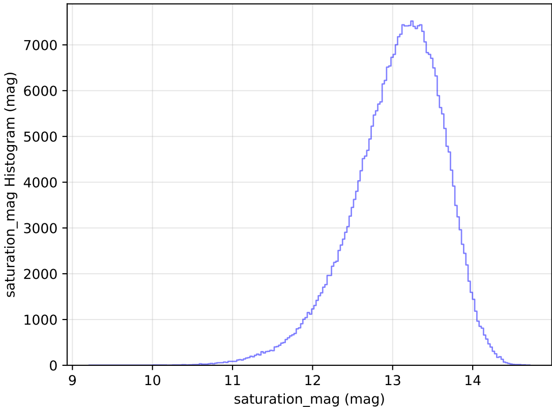
smc_lmc_v3.3_10yrs WFD y band: saturation_mag Histogram
