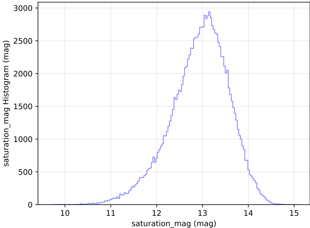
smc_lmc_v3.3_10yrs WFD u band: saturation_mag Histogram
