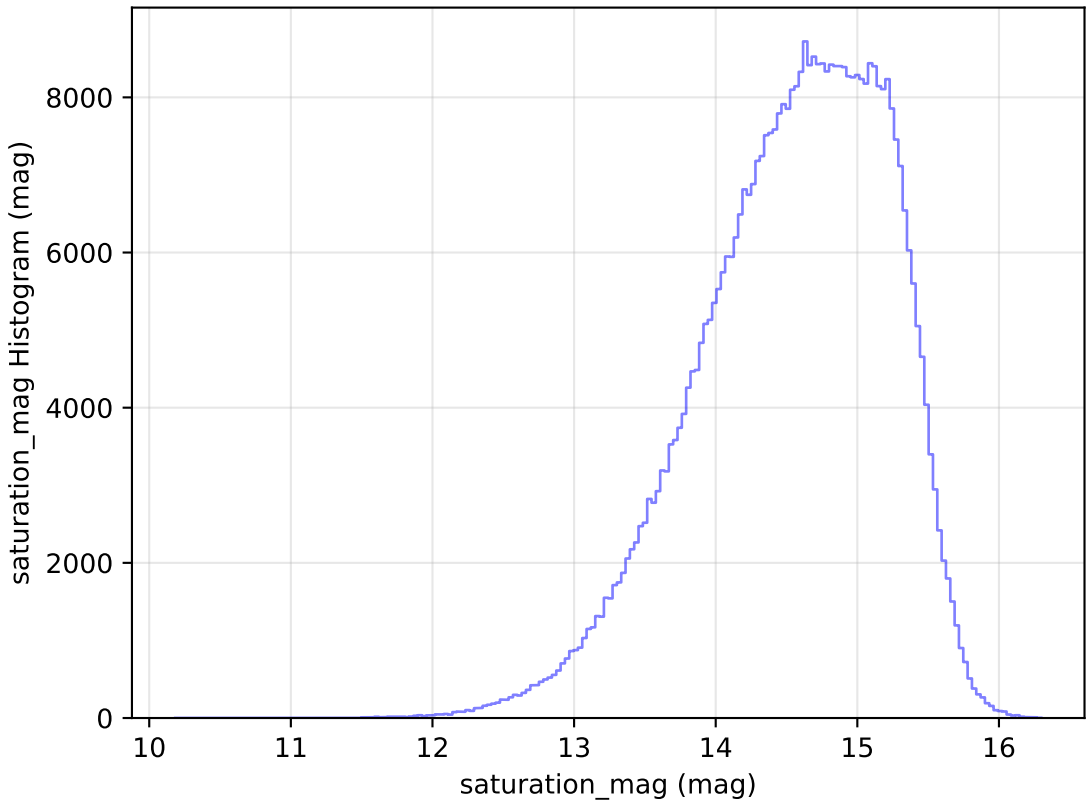
smc_lmc_v3.3_10yrs WFD r band: saturation_mag Histogram
