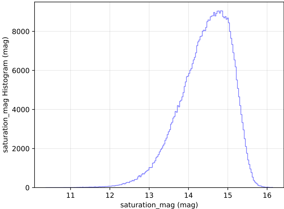
smc_lmc_v3.3_10yrs WFD i band: saturation_mag Histogram
