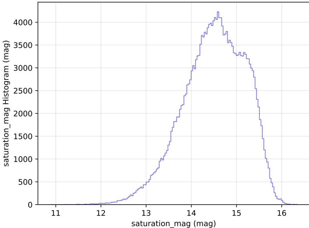
smc_lmc_v3.3_10yrs WFD g band: saturation_mag Histogram
