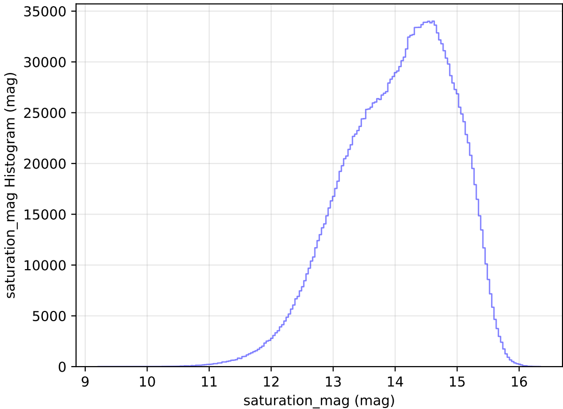
smc_lmc_v3.3_10yrs WFD all bands: saturation_mag Histogram
