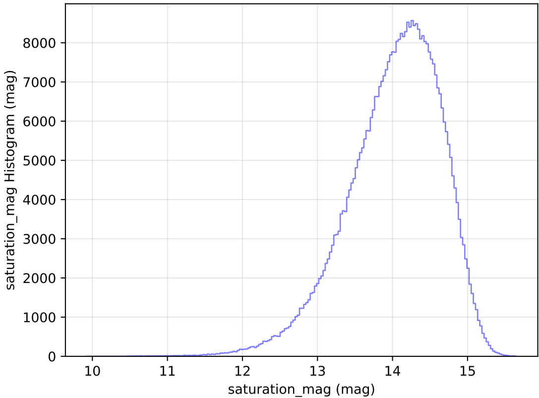
smc_lmc_v3.3_10yrs All sky z band: saturation_mag Histogram
