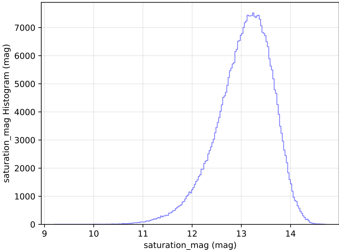
smc_lmc_v3.3_10yrs All sky y band: saturation_mag Histogram
