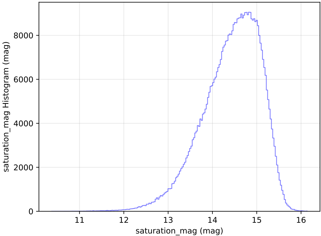
smc_lmc_v3.3_10yrs All sky i band: saturation_mag Histogram
