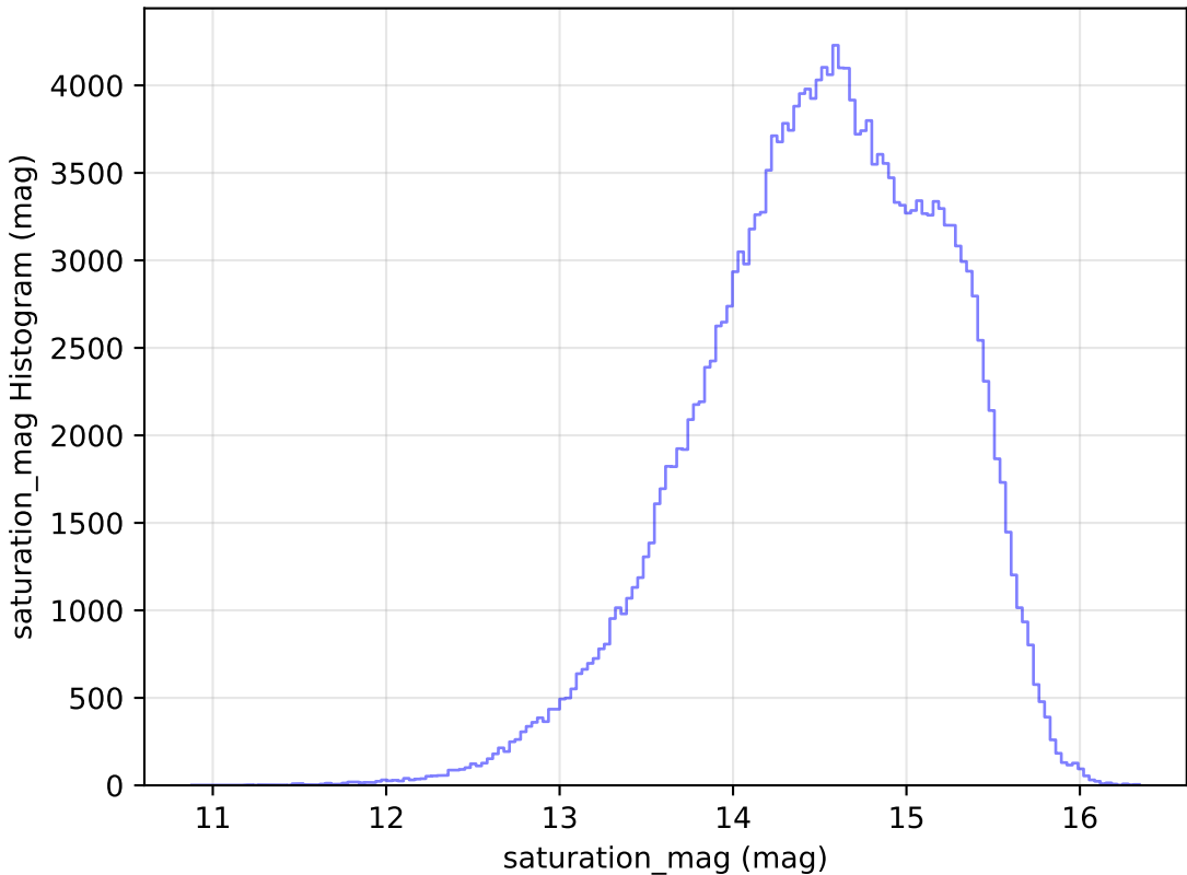
smc_lmc_v3.3_10yrs All sky g band: saturation_mag Histogram
