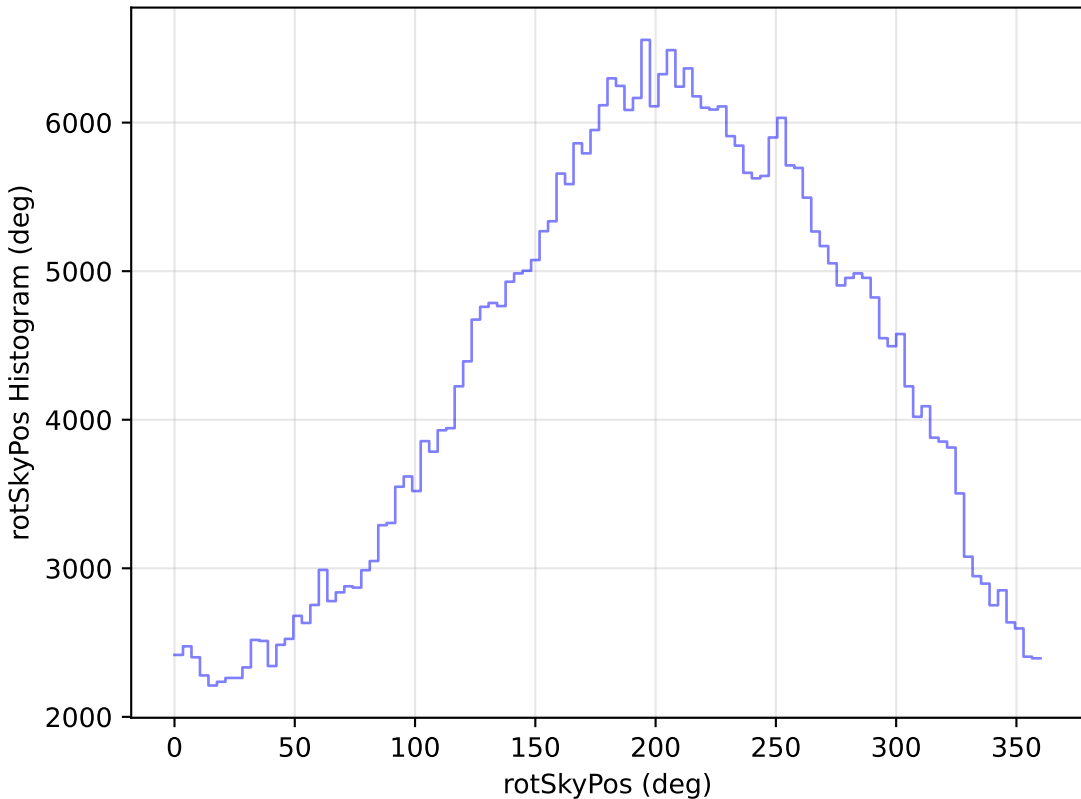
smc_lmc_v3.3_10yrs WFD z band: rotSkyPos Histogram
