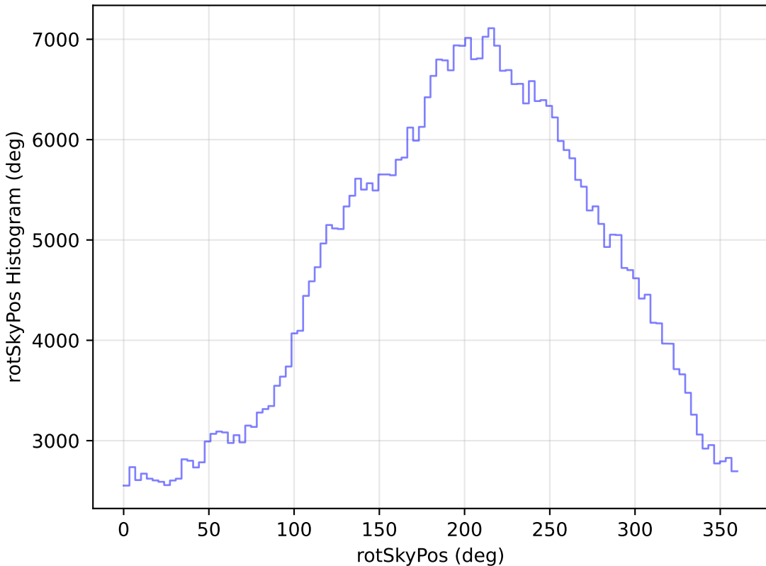
smc_lmc_v3.3_10yrs WFD i band: rotSkyPos Histogram
