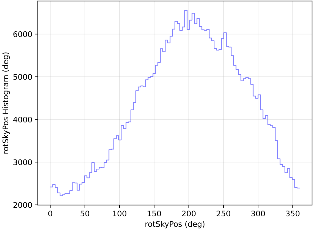
smc_lmc_v3.3_10yrs All sky z band: rotSkyPos Histogram
