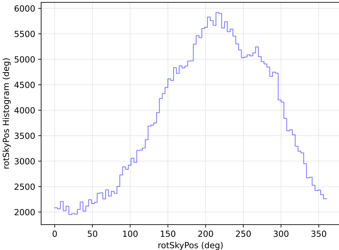
smc_lmc_v3.3_10yrs All sky y band: rotSkyPos Histogram
