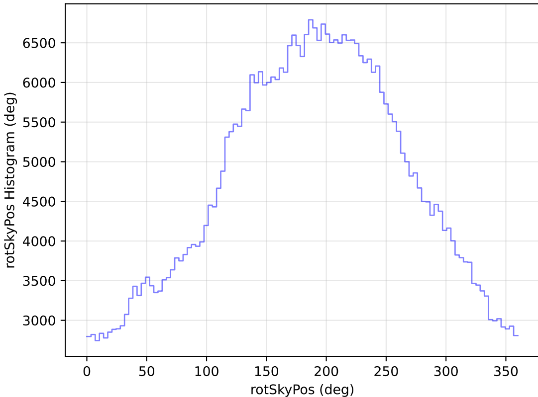
smc_lmc_v3.3_10yrs All sky r band: rotSkyPos Histogram
