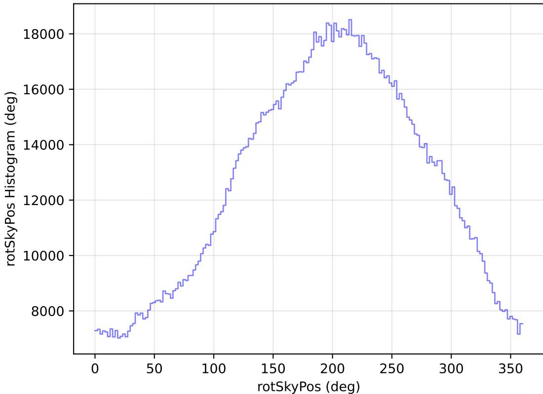
smc_lmc_v3.3_10yrs All sky all bands: rotSkyPos Histogram
