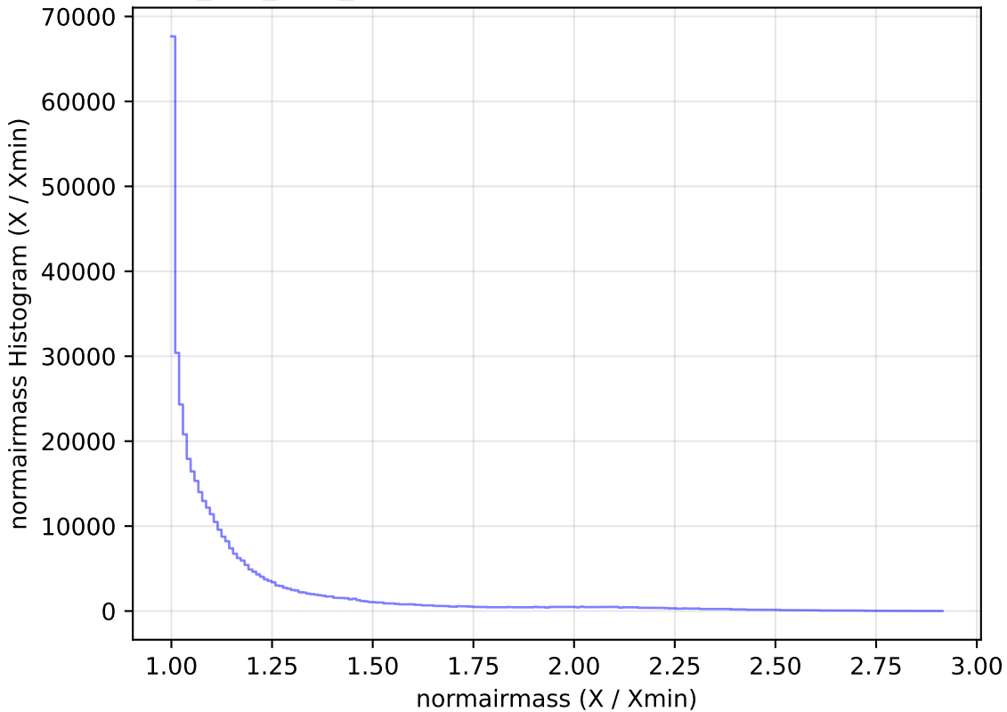
smc_lmc_v3.3_10yrs WFD z band: normairmass Histogram
