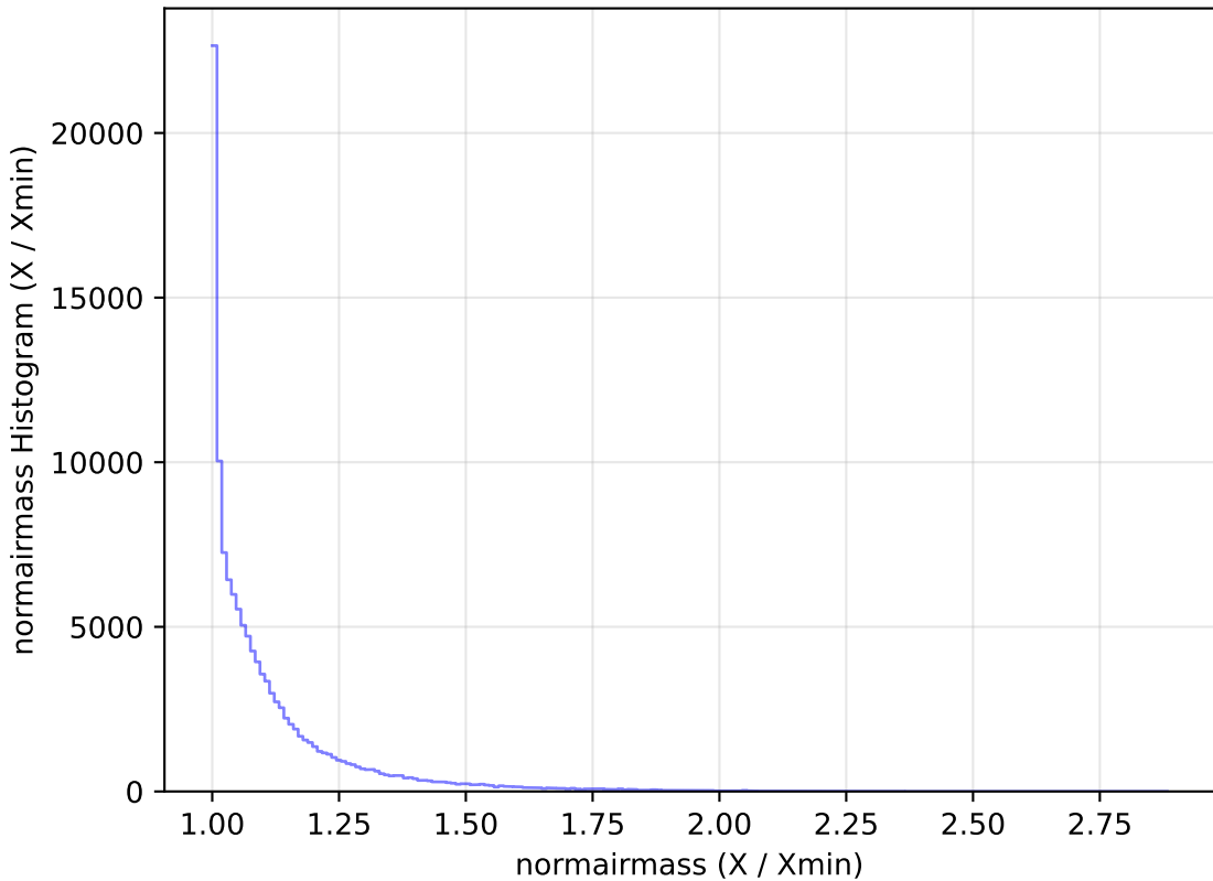
smc_lmc_v3.3_10yrs WFD u band: normairmass Histogram
