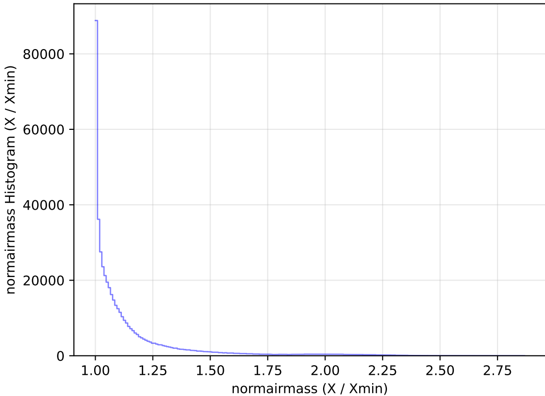
smc_lmc_v3.3_10yrs WFD r band: normairmass Histogram
